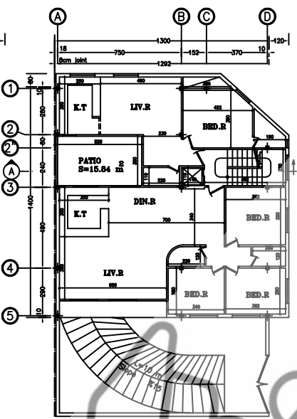
1ST. & 2ND. FLOOR PLAN SCALE 1:100
