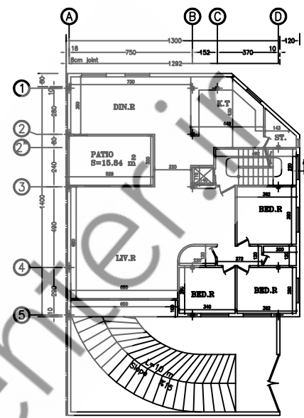
TYPICAL PLAN SCALE 1:100
