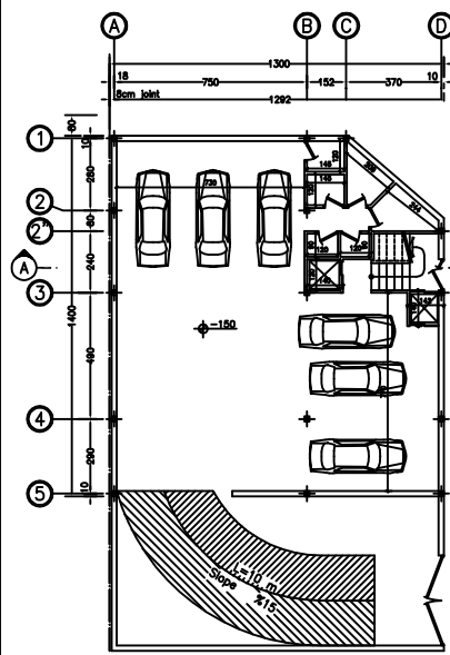
BASEMENT PLAN SCALE 1:100
