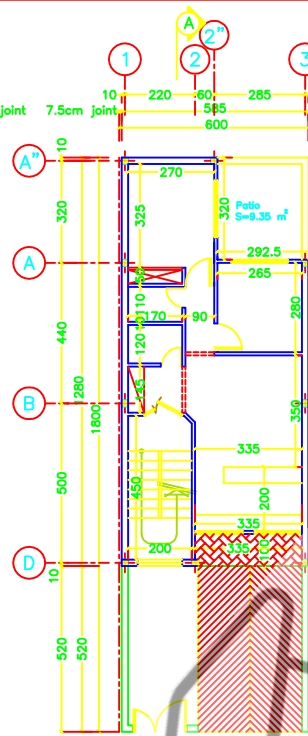
TYPICAL FLOOR PLAN SCALE 1:100
