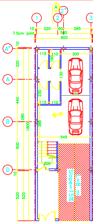
BASEMENT FLOOR PLAN SCALE 1:100
