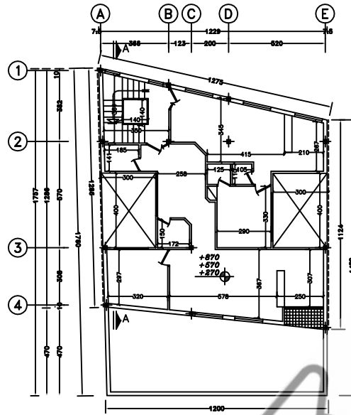
(1&2&3TH) FLOOR PLAN SC. 1:100
