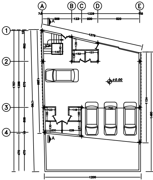
GROUND FLOOR PLAN SC. 1:100
