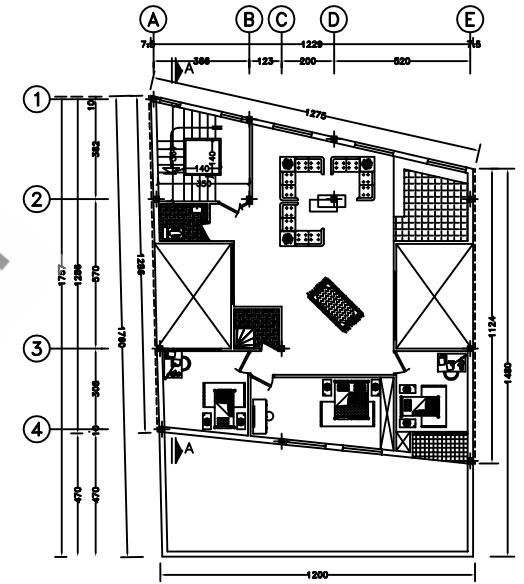
FURNITURE PLAN SC. 1:100
