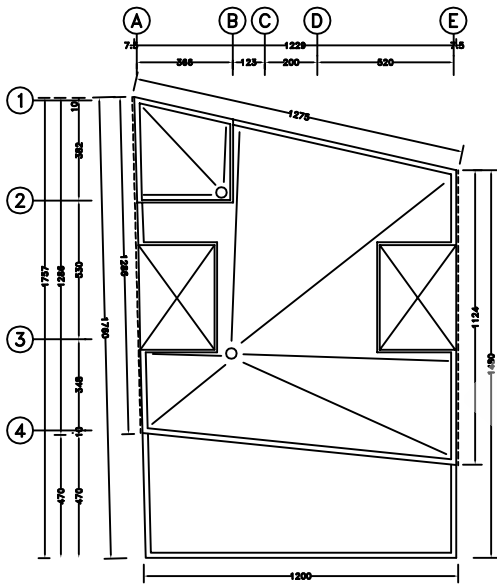
ROOF PLAN SC. 1:100
