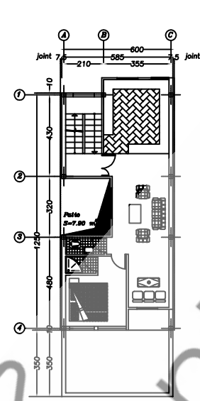
DECORATION PLAN SC. 1:100
