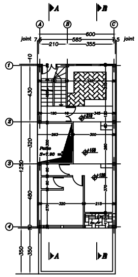
GROUND FLOOR PLAN SC. 1:100
