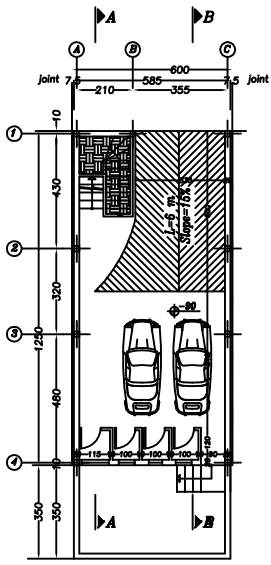
BASEMENT PLAN SC. 1:100
