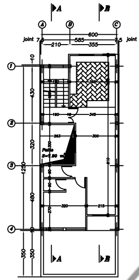
TYPICAL FLOOR PLAN SC. 1:100
