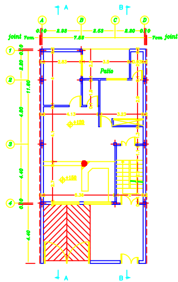
GROUND FLOOR PLAN SC: 1:100
