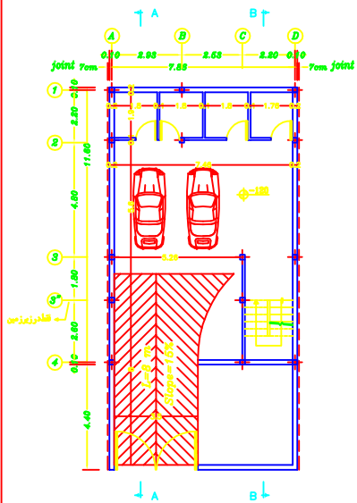
BASEMENT FLOOR SC: 1:100
