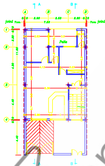
TYPICAL FLOOR PLAN SC: 1:100
