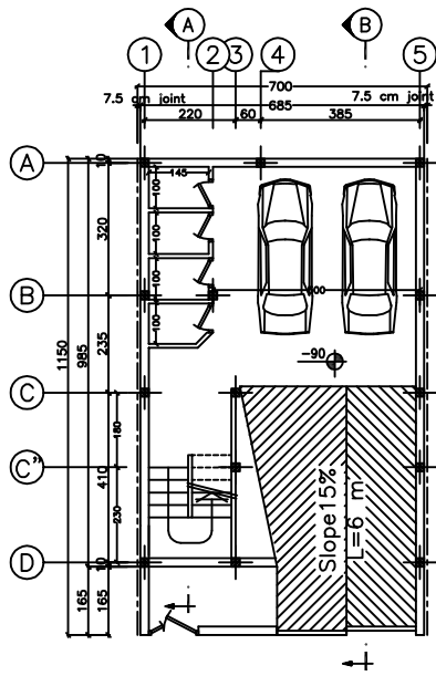
BASEMENT FLOOR PLAN SCALE 1:100
