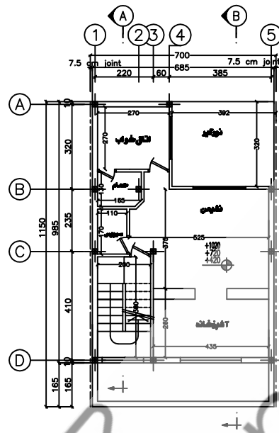
TYPICAL FLOOR PLAN SCALE 1:100
