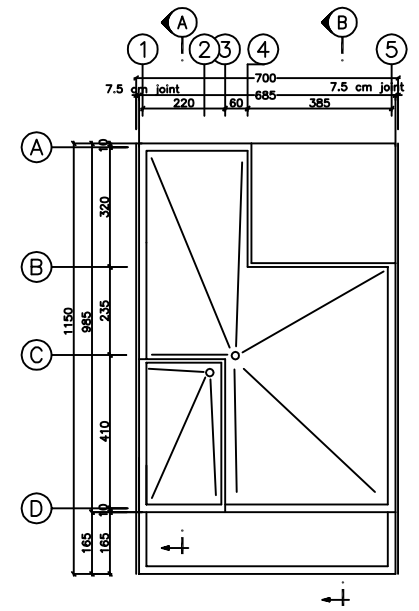
ROOF PLAN SCALE 1:100
