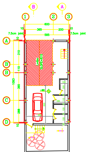
BASEMENT PLAN SC. 1:100
