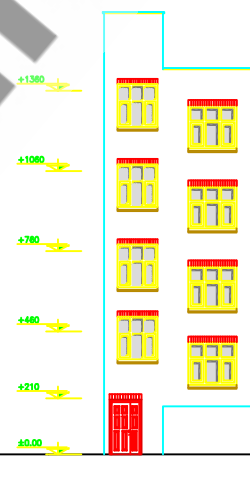
NORTH ELEVATION SC. 1:100
