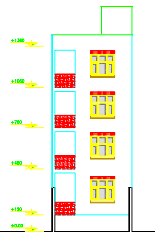
SOUTH ELEVATION SC. 1:100
