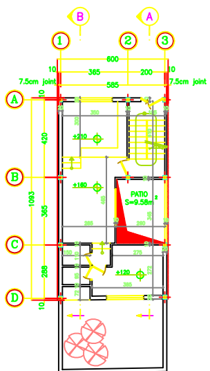
FIRAT FLOOR PLAN SC. 1:100
