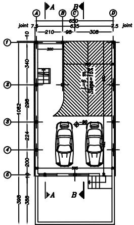
BASEMENT PLAN SC. 1:100
