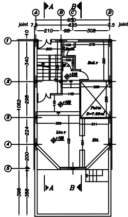
GROUND FLOOR PLAN SC. 1:100
