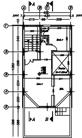
TYPICAL FLOOR PLAN SC. 1:100
